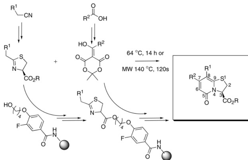
FIGURE 2. Synthetic methods toward substituted bicyclic 2-pyridones based upon the acyl-ketene imine cycloaddition. 7–9
