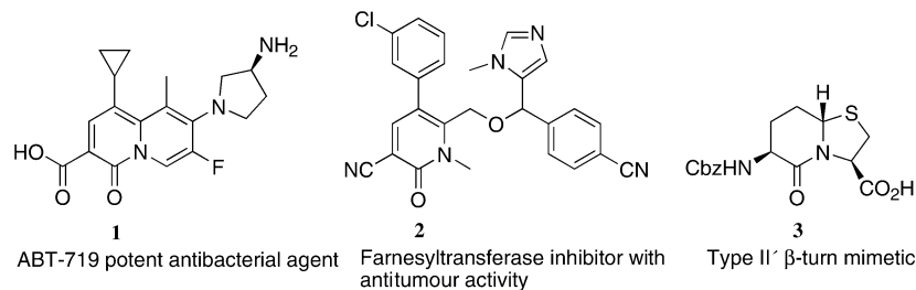
FIGURE 1. Examples of 2-pyridones ( 1 and 2 ) and a tetrahydro derivative 3 with different biological effects. 1,4,14
